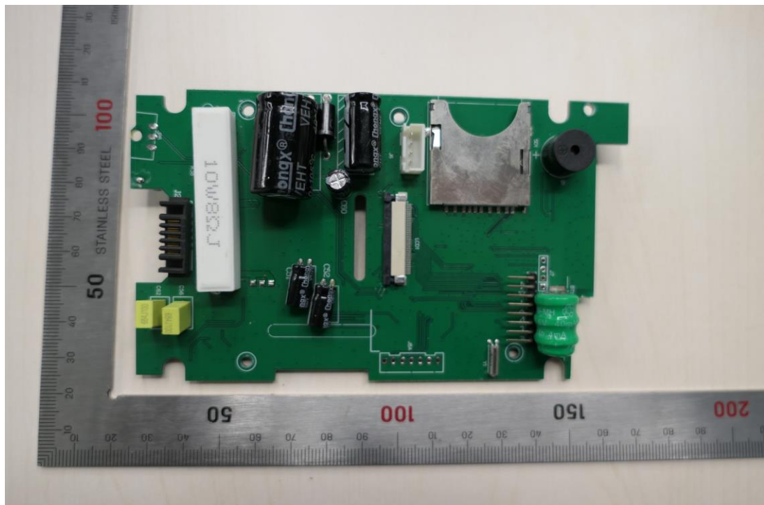
Figure 10 Main board-2
