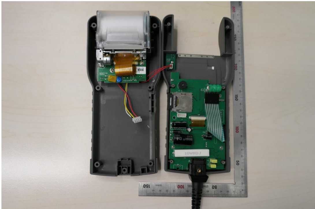
Figure 6 Internal view
