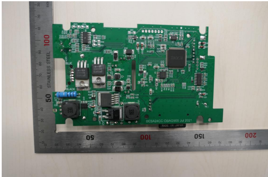
Figure 9 Main board -1
